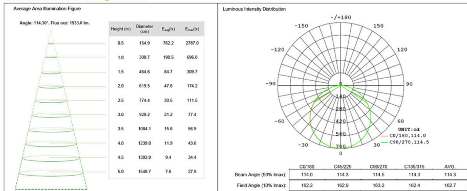
8 Inch, 24W LED DOWN LIGHT @ 220V 50Hz
